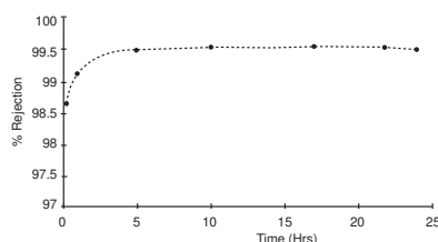
Figure 1. Stabilized salt rejection performance of FILMTEC elements after system startup
